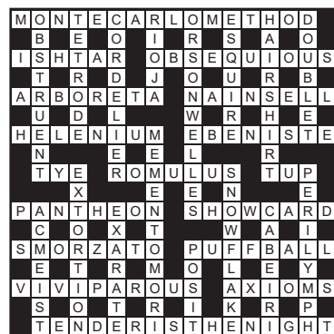
Solution Polymath 1,184
