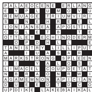
Solution Polymath 1,159
