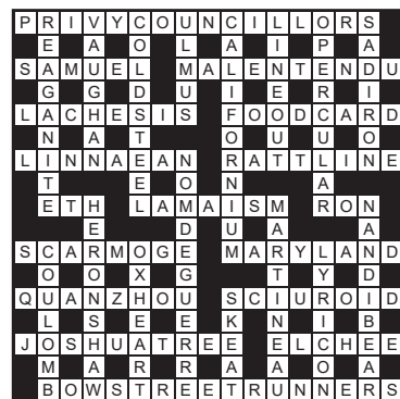
Solution Polymath 1,114
