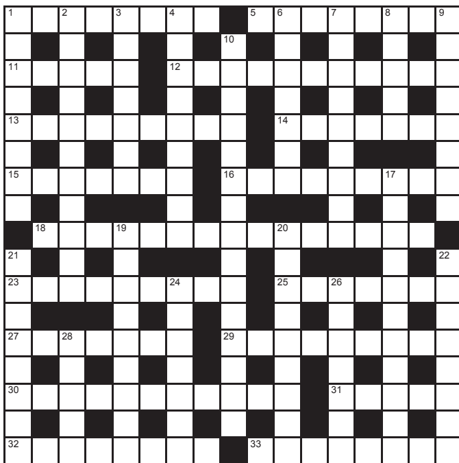
Solution Polymath 1,114
